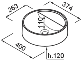
Technical Drawing
